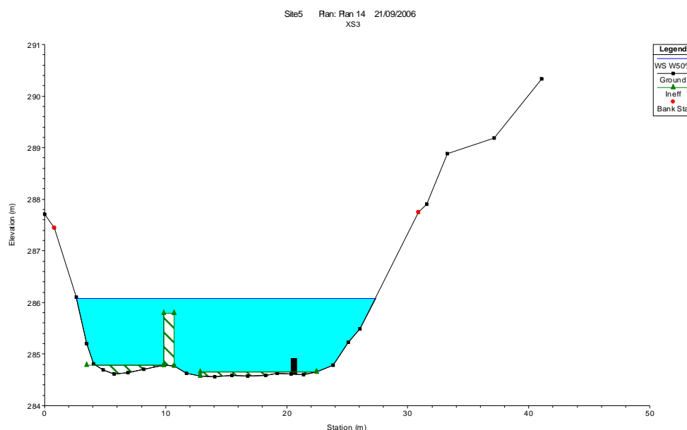
■ Figure 3-74: Water level at cross-section 3 at study site, Reach 5, under winter fresh of 700 ML/day.
