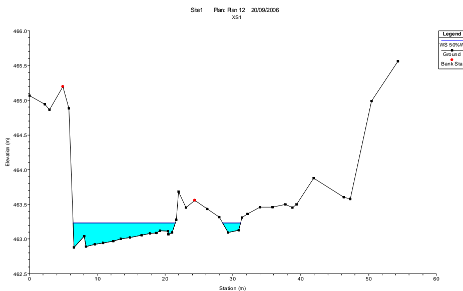
■ Figure 3-14: Water depth at cross-section 1, at the study site, Reach 1, under a winter fresh of 294 ML/day.
