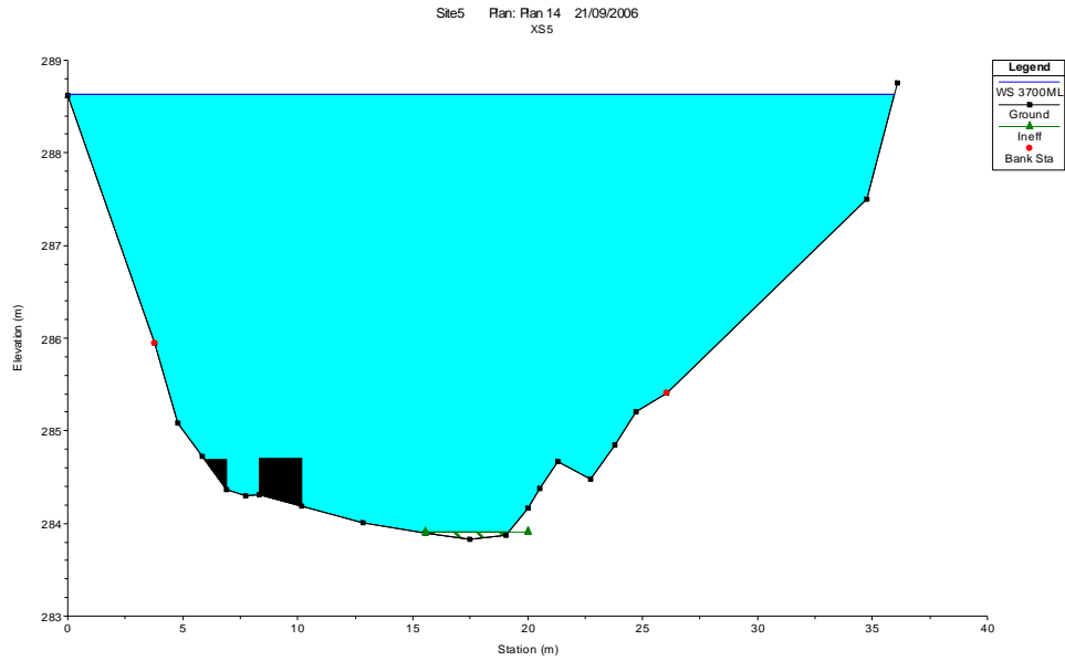
■ Figure 3-76: Water level at cross-section 5 at study site, Reach 5, under winter high flow of 3700 ML/day.
