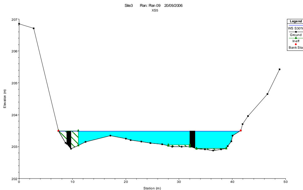
■ Figure 3-37: Water level at cross-section 5, at study site Reach 3 under a summer fresh of 595 ML/day.
