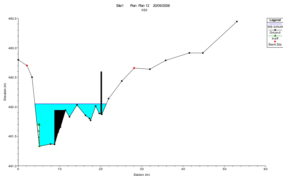
■ Figure 3-13: Water level at cross-section 5, at the study site, Reach 1, under a winter fresh of 294 ML/day.
