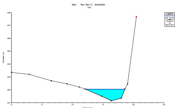
■ Figure 3-7: Water level at cross-section 4, at study site, Reach 1, under a summer fresh of 95 ML/day. Note water level in photograph does not necessarily reflect level shown in cross section.
