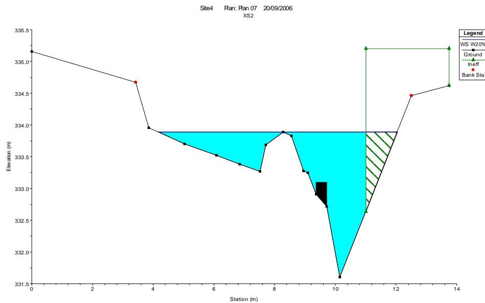
■ Figure 3-60: Water level, cross-section 2 at study site, Reach 4, under winter high flow of 383 ML/day.
