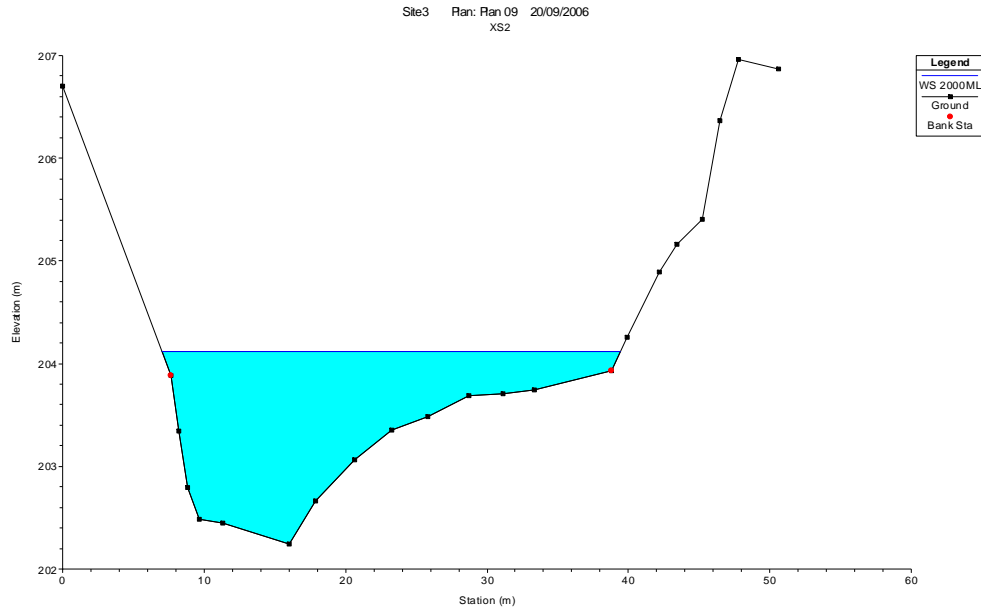
■ Figure 3-39: Water level at cross-section 2, at study site, Reach 3, under a summer high flow of 2000 ML/day.
