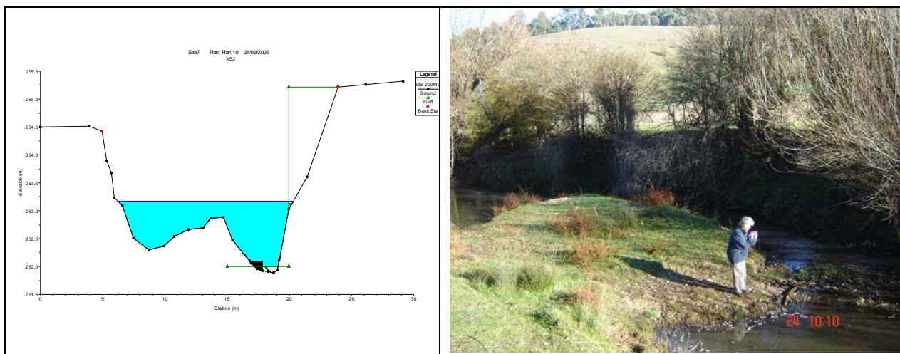
■ Figure 3-84: Water level at cross-section 2 at study site, Reach 7, under summer high flow of 200 ML/day. Note water level in photograph does not necessarily reflect level shown in cross section.
