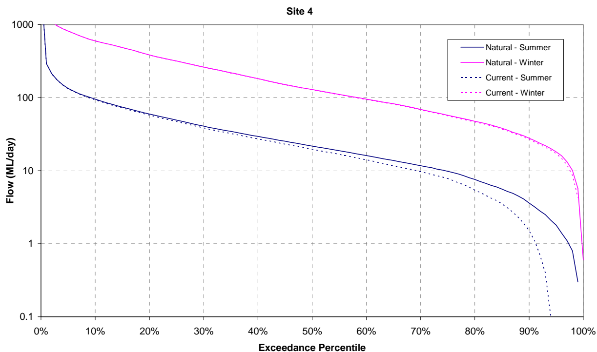
■ Figure 3-49: Natural and Current summer and winter percentage exceedance curves for Site 4.
