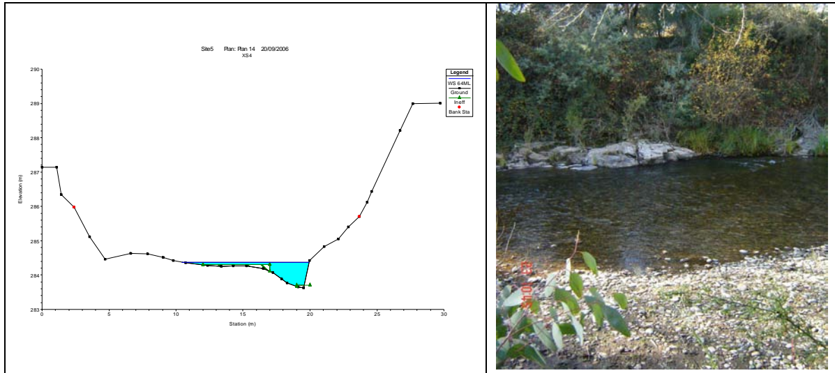
■ Figure 3-65: Water level at cross-section 4 at study site, Reach 5, under summer low flow of 64 ML/day. Note water level in photograph does not necessarily reflect level shown in cross section.
