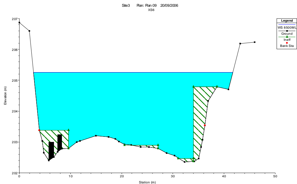
■ Figure 3-47: Water level at cross-section 6, at this site, Reach 3, under winter high flow of 8500 ML/day.
