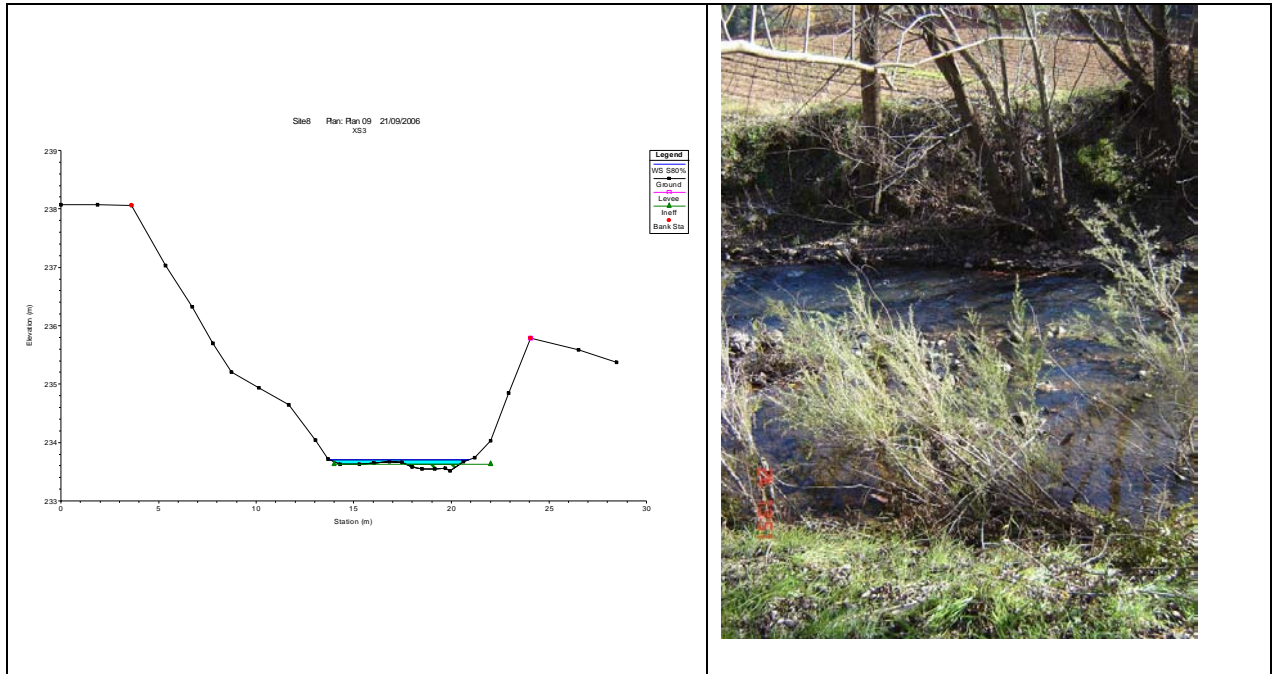
■ Figure 3-93: Water level at cross-section 3 at study site, Reach 8, under summer low flow of 15 ML/day. Note water level in photograph does not necessarily reflect level shown in cross section.
