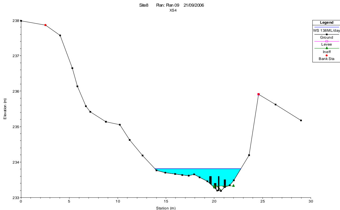
■ Figure 3-101: Water level at cross-section 4 at study site, Reach 8, under winter fresh of 138 ML/day.
