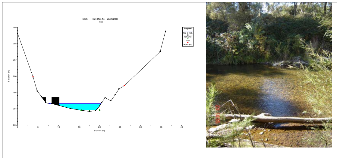
■ Figure 3-66: Water level at cross-section 5 at study site, Reach 5, under summer low flow of 64 ML/day. Note water level in photograph does not necessarily reflect level shown in cross section.
