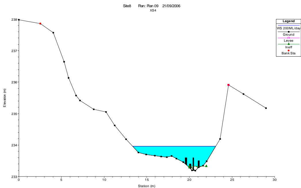
■ Figure 3-97: Water level at cross-section 4 at study site, Reach 8, under summer high flow of 200 ML/day.
