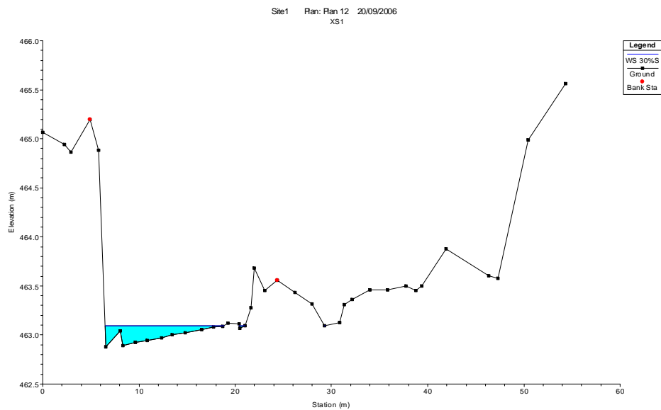
■ Figure 3-6: Water level at cross-section 1, at study site in Reach 1 under a summer fresh of 95 ML/day.
