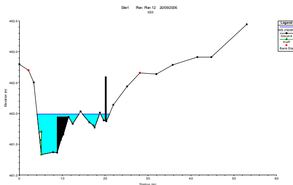
■ Figure 3-9: Water levels at cross-section 5, at study site, Reach 1, under a summer high flow of 250 ML/day. Note water level in photograph does not necessarily reflect level shown in cross section.
