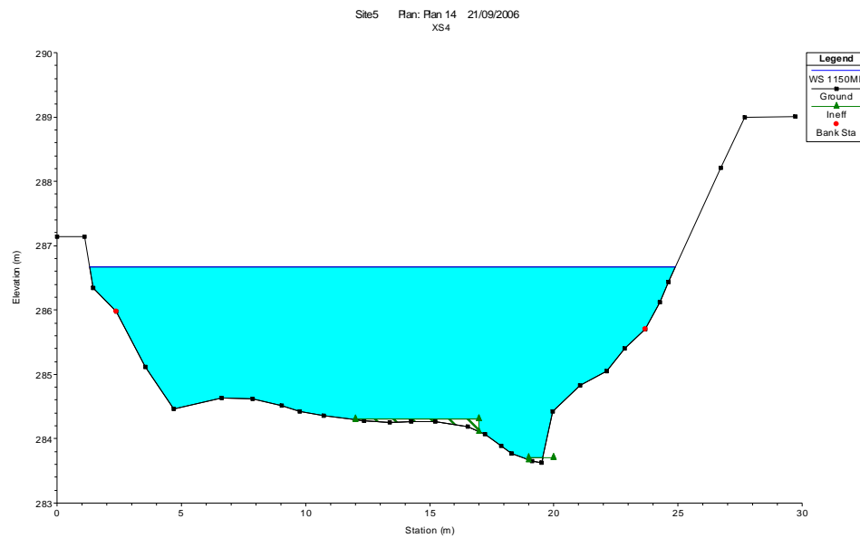
■ Figure 3-70: Water level at cross-section 4 at study site, Reach 5, under summer high flow of 1150 ML/day.
