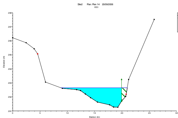
Figure 3-29: Water level at cross-section 3, at study site, Reach 2, under a winter fresh of 677 ML/day. Note water level in photograph does not necessarily reflect level shown in cross section.
