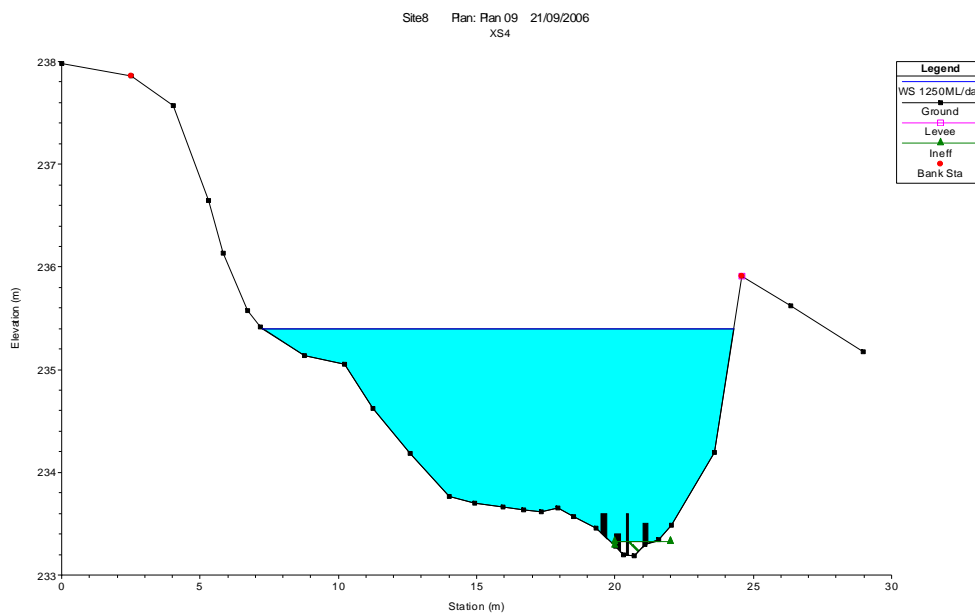
■ Figure 3-103: Water level at cross-section 4 at study site, Reach 8, under winter high flow of 1250 ML/day.
