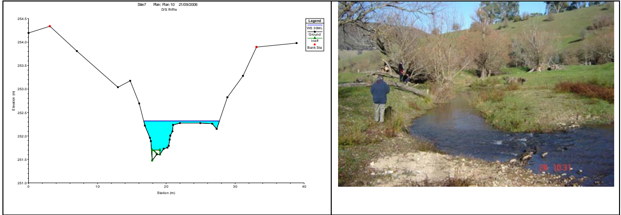
■ Figure 3-82: Water level at cross-section upstream of cross-section 7, at study site, Reach 7 under summer fresh of 35 ML/day. Note water level in photograph does not necessarily reflect level shown in cross section.
