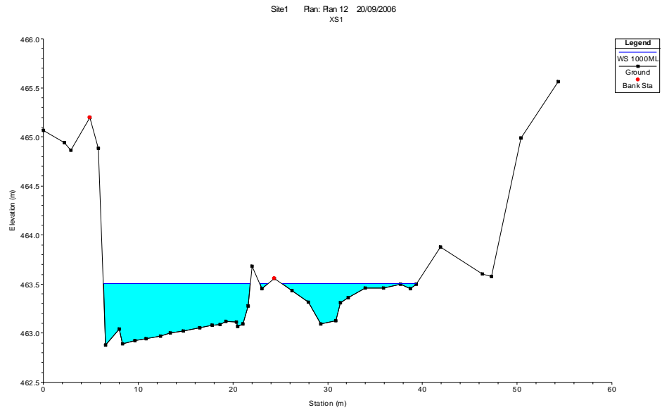
■ Figure 3-16: Water level at cross-section 1, at study site, Reach 1, for a winter high flow (winter high flow 1) of 1000 ML/day.
