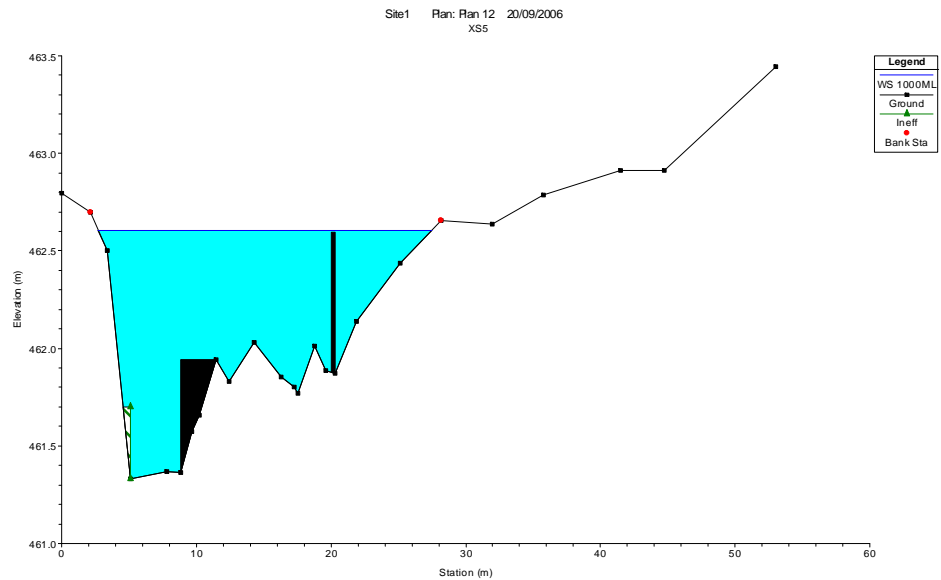
■ Figure 3-17: Water level at cross-section 5, at study site, Reach 1, for a winter high flow (winter high flow 1) of 1000 ML/day.
