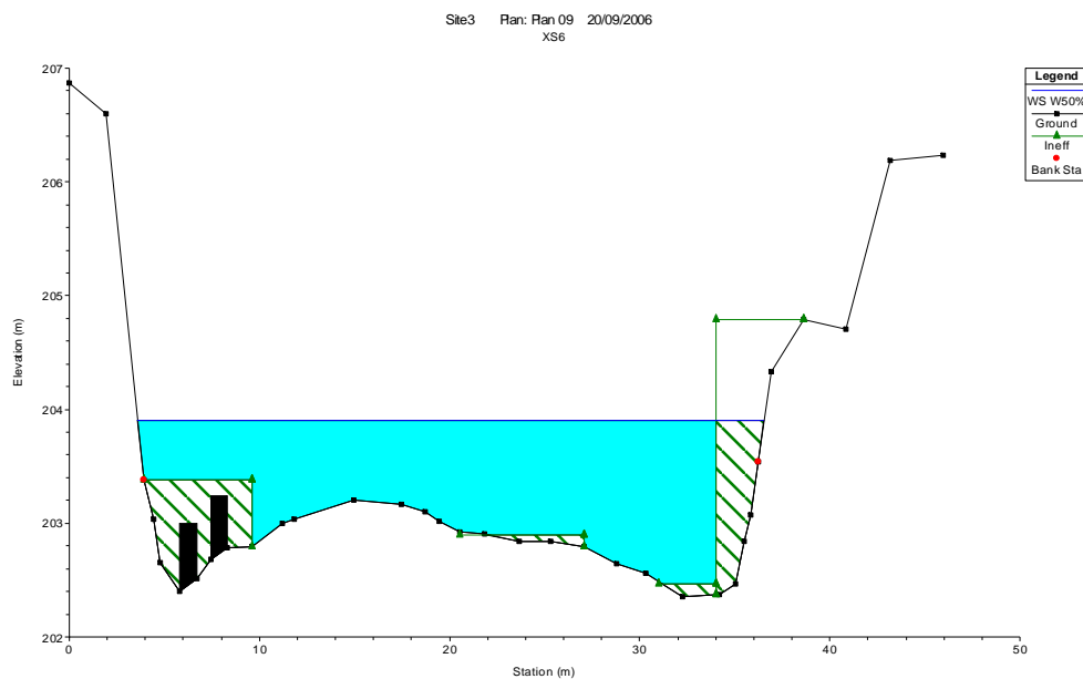
■ Figure 3-45: Water level at cross-section 6, at study site, Reach 3, under winter fresh of 1870 ML/day.
