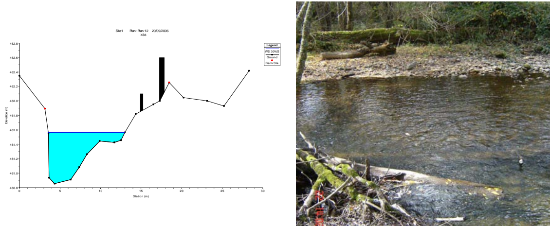
■ Figure 3-5: Water depth at cross-section 6, at study site, Reach 1, under a summer fresh of 95 ML/day. Note water level in photograph does not necessarily reflect level shown in cross section.
