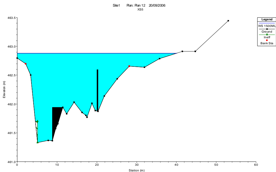
■ Figure 3-20: Water level at cross-section 5, at study site, Reach 1, under a winter high flow (winter high flow 2) of 1500 ML/day.
