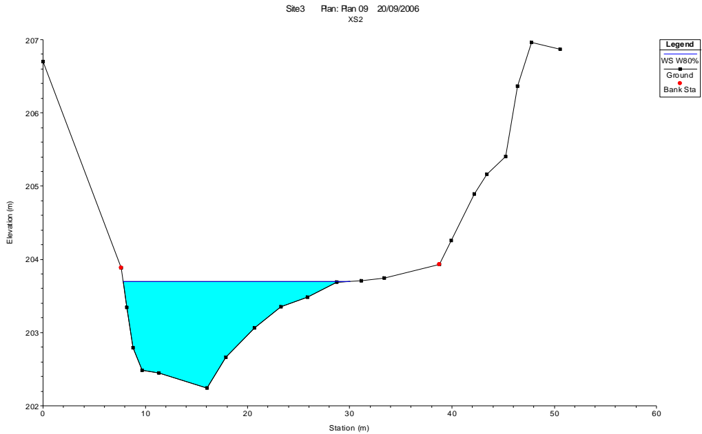
■ Figure 3-42: Water level at cross-section 2, at study site, Reach 3, under winter low flow of 740 ML/day.
