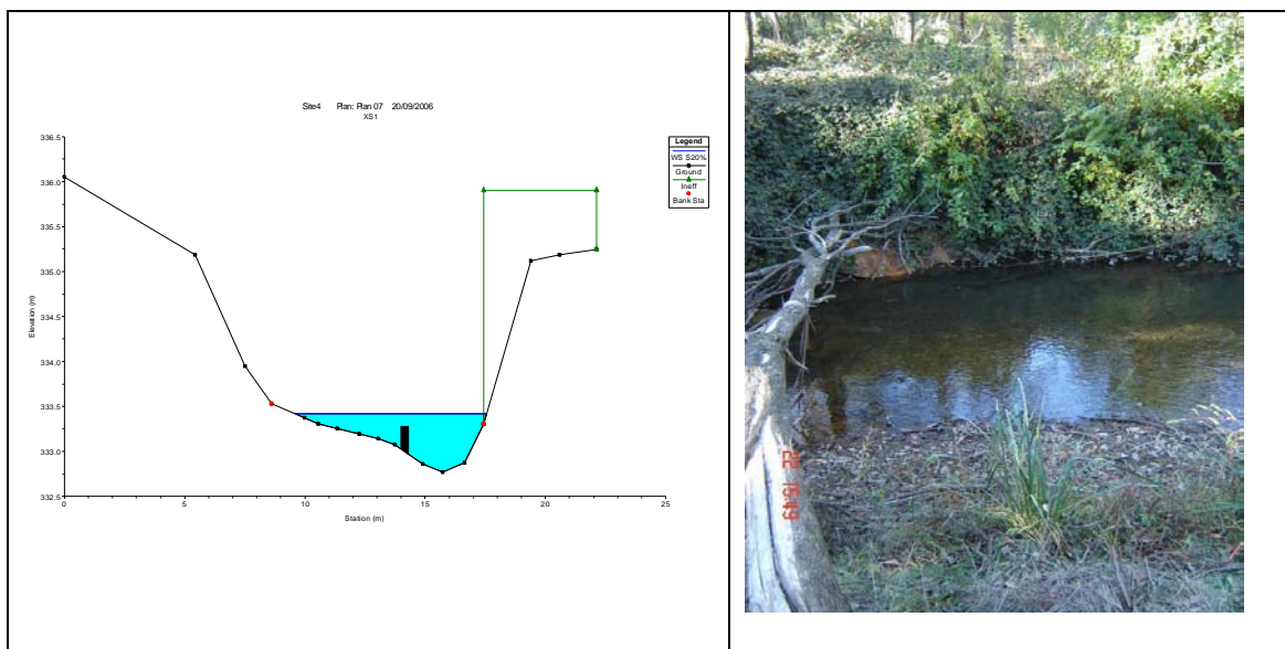
■ Figure 3-52: Water level at cross-section 1 at study site, Reach 4, under summer fresh of 60 ML/day. Note water level in photograph does not necessarily reflect level shown in cross section.
